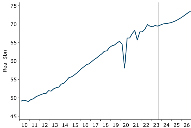
Figure 4. OCR forecast
